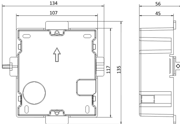
Figure 2-7 Front and Side View of the Gang Box
